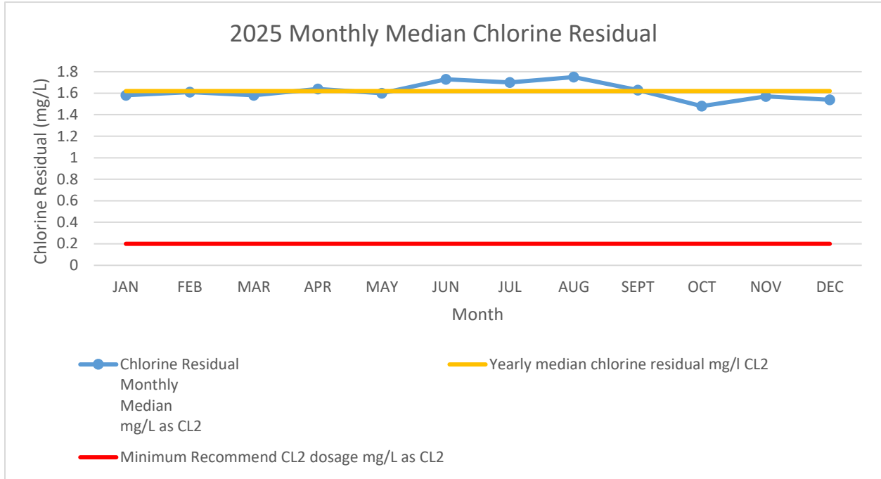
Figure 1 - 2025 Monthly Median Chlorine Residual
